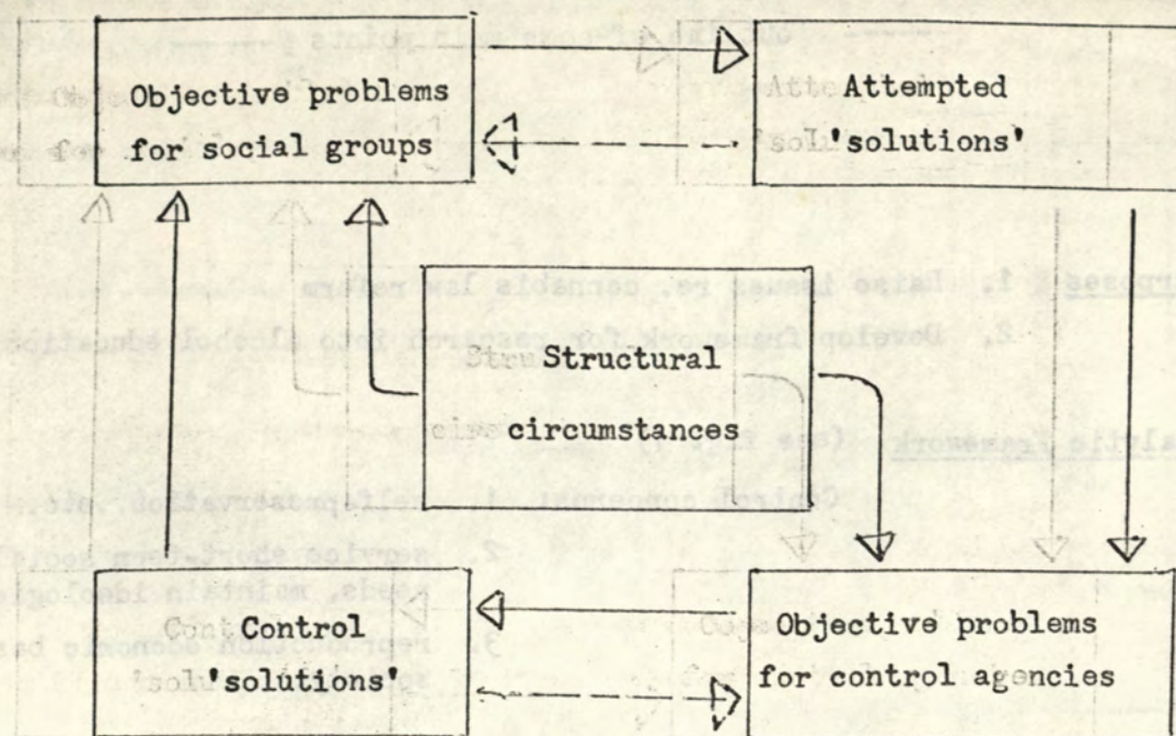
FIGURE 1: Analytic Framework
